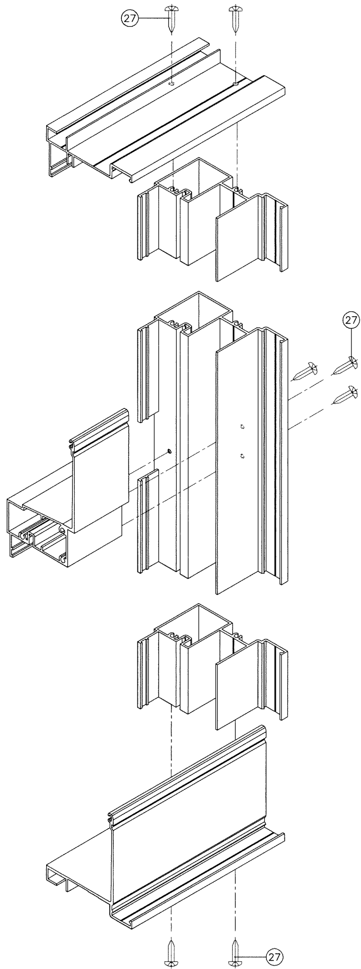
FRAME CORNERS DETAIL
