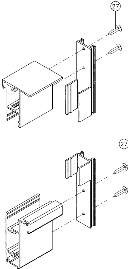
VENT CORNER DETAIL
